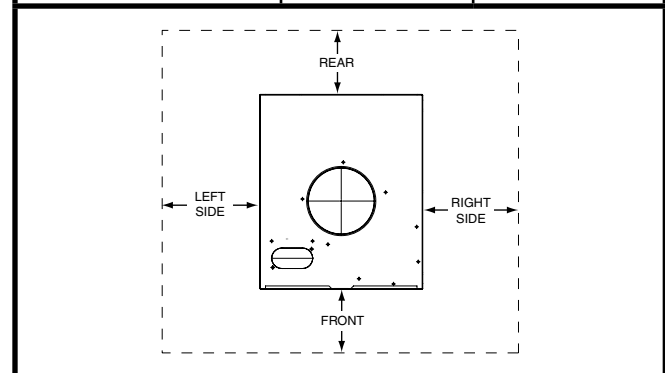
Figure 1. Minimum Clearances
