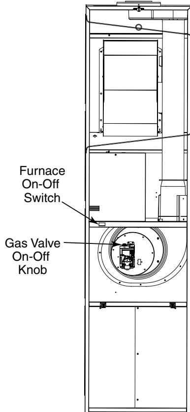
Figure 2. MG1 Gas Furnace Components
